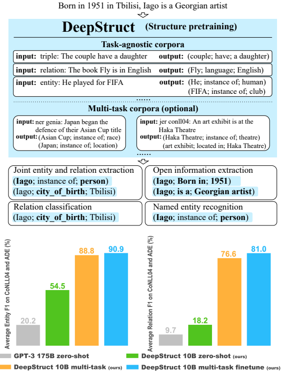
Figure 1: Summary of our approach and results. Upper: an overview of DEEPSTRUCT and the proposed structure pretraining. Lower: performance of our 10B DEEPSTRUCT zero-shot and multi-task, compared with 175B GPT-3 zero-shot.
