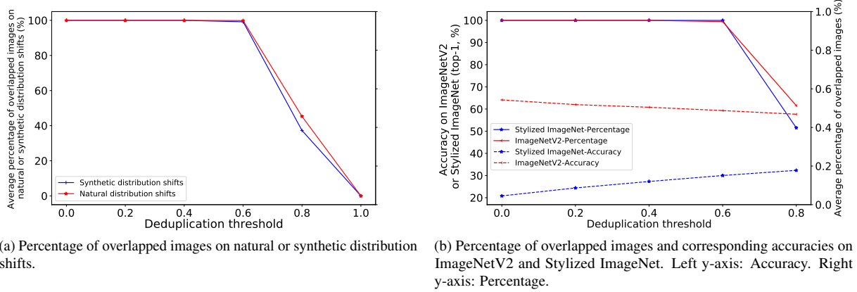
Figure 6. Data overlap between YFCC100M (pre-training data) and distribution shifts.
