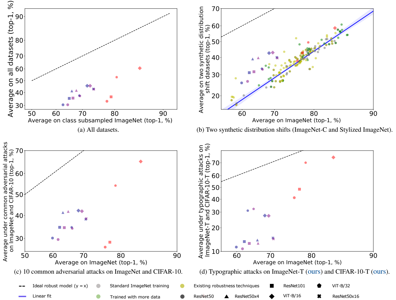
Figure 2. Zero-shot multimodal CLIP fails to significantly improve the robustness over standard ImageNet models on our RoZ benchmark. Red: standard ImageNet models. Blue: zero-shot CLIP models. Purple: CLIP-Auto models. The notable outlier to this trend is CLIP on natural distribution shifts. In particular, we observe a significant performance drop in robustness on our ImageNet-T and CIFAR-10-T. The original CLIP and CLIP-Auto perform similarly on all the test sets.
